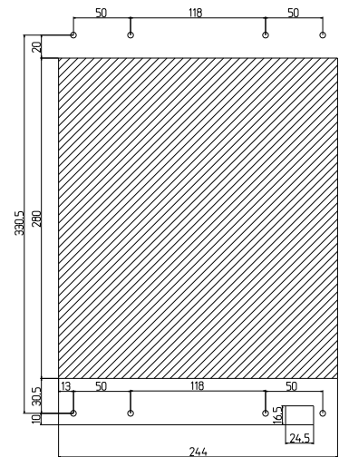
Ⓑ Enclosure mounting
