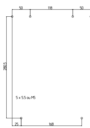
Ⓐ Rear mounting
